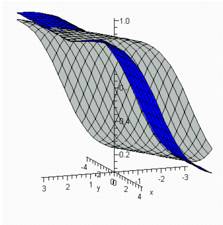
Figure 12. An Example of Item Characteristics Surface for the Focal Group and the Reference Group Using MAPLE
