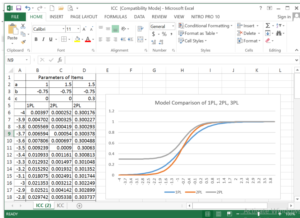
Figure 1. Model Comparison in Unidimensional Item Response Theory
