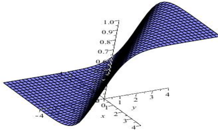
Figure 9. An Example of Item Characteristic Surface that Measured 2 Dimensions
