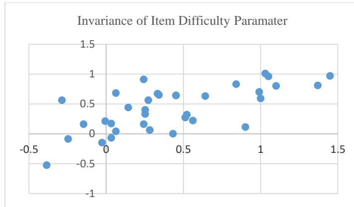
Figure 5. An Example of Scatterplot for Proving the Parameter Invariance
