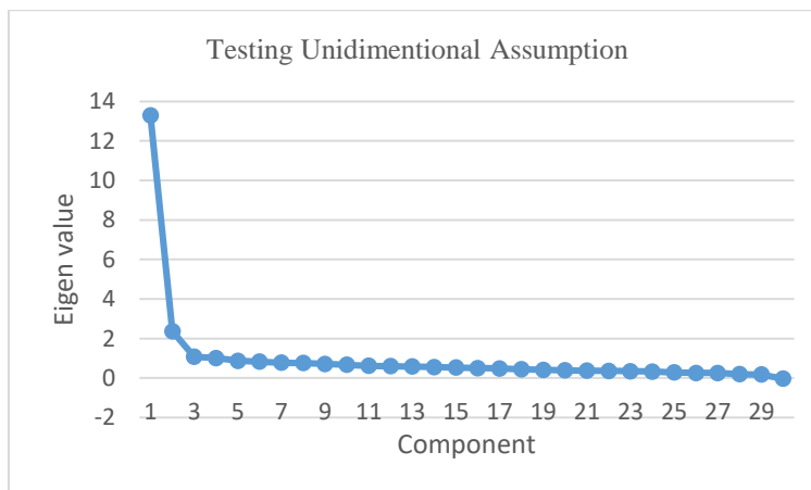
Figure 4. An Example of Scree-Plot for Proving the Unidimension
