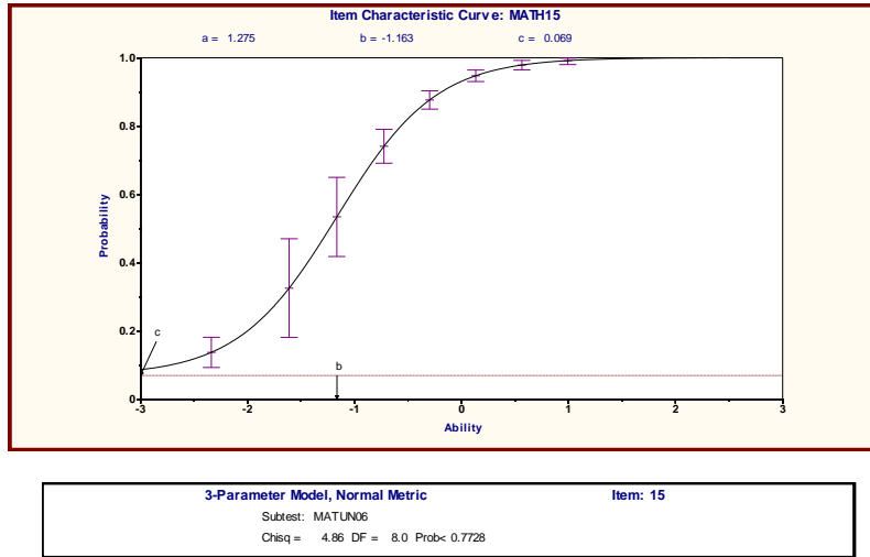
Figure 3. An Example of Output Results from the Analysis Using 3PL Model with BILOGMG
