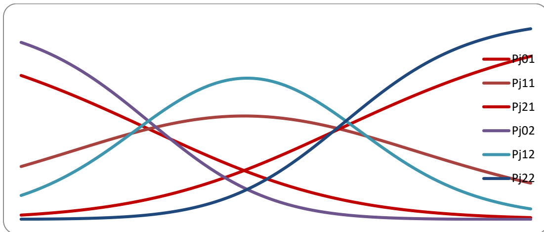
Figure 11. An Example of Category Response Function for the Focal Group and the Reference Group
