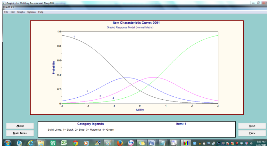
Figure 7. An Example of Output from the Item Category Response Function with GRM-Type
