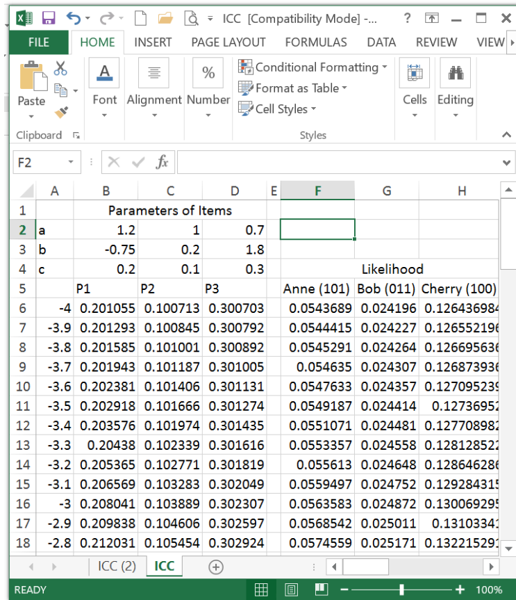
Figure 2. An Example of Worksheet of Ability Parameters Estimation with Maximum Likelihood
