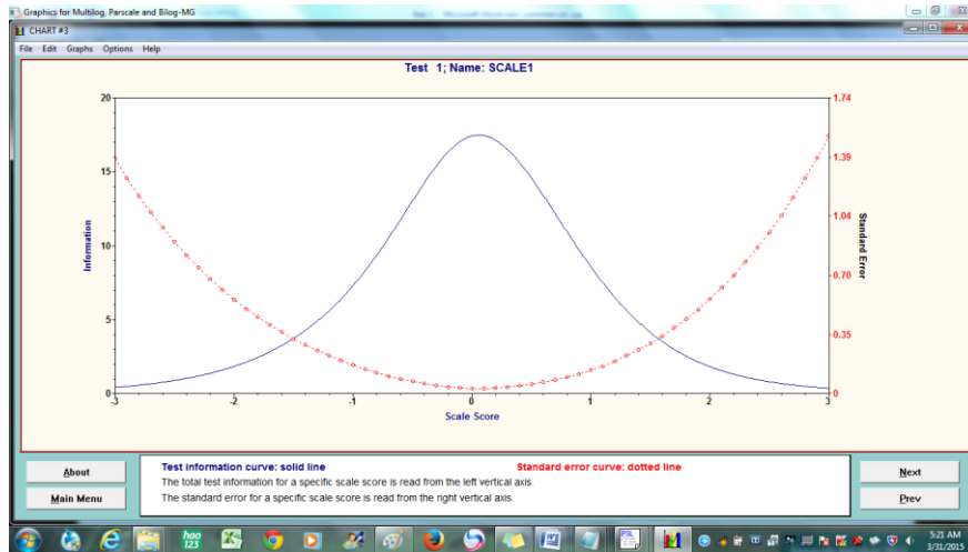
Figure 8. An Example of Output from the Value of Item Information Function and Measurement Errors
